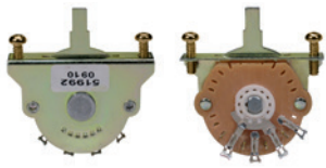
Oak Grigsby lever switch 3-way, bolts included, no cap 31549 SW-OAK-3 single switch 31737 SW-OAK-3/12 bulk pack 12 pcs
