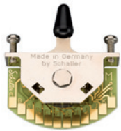
Schaller Megaswitch, 40,7mm spacing, bolts included, black cap 42535 15310002 E lever switch 5-way 42536 15310003 S lever switch 5-way 42537 15310006 M lever switch 5-way 42538 15310013 T lever switch 3-way
