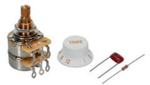
Fender Genuine Replacement Part TBX Tone potentiometer 33911 0992052000 standard length bushing .375", 3/8" diameter, with .022mf capacitor
