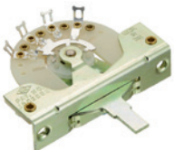
Fender Genuine Replacement Part CRL 5-way lever switch for strat/tele 43365 0038929049
